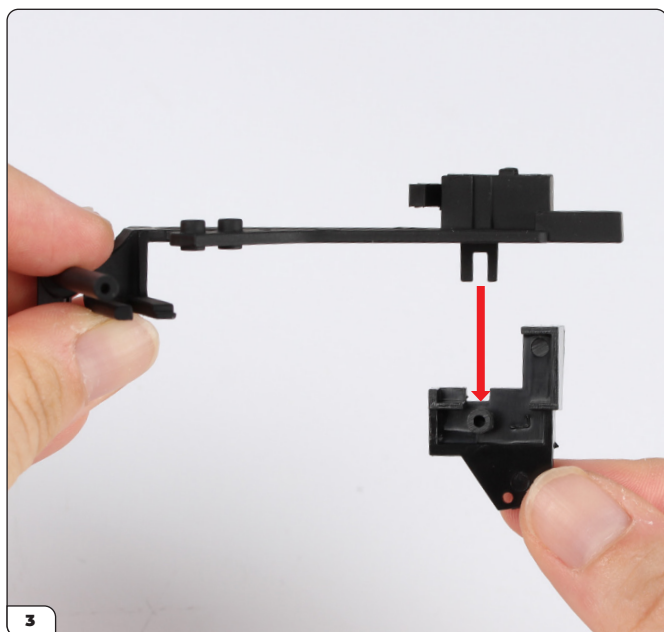
Push mechanism part 1 into mechanism part 3 (98-C) in the orientation shown.
