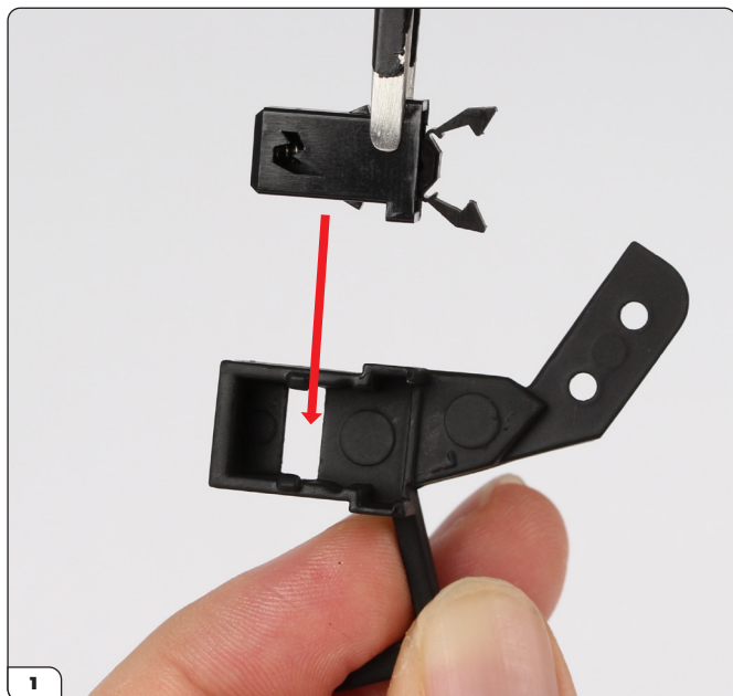
Assembling the Headlight Minigun Mechanism Press one of the clamps (98-H) into the mechanism part 2 (98-B).
