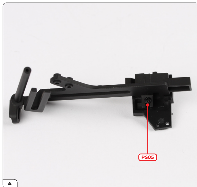
Screw the parts together with a PS05 screw.
