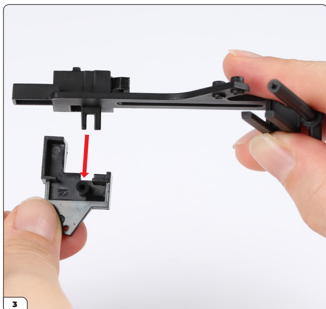
Push mechanism part 1 into mechanism part 3 (96-C) in the orientation shown.
