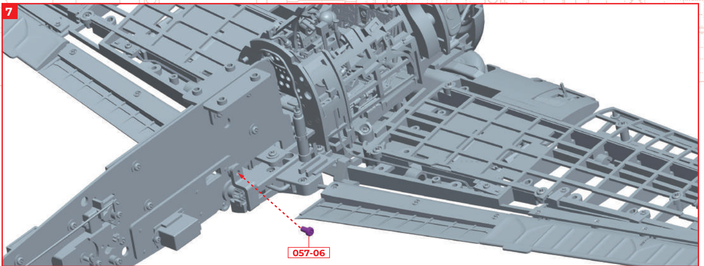
Fix the gear cover 057-02 in place with the screw 057-06 that came with stage 57.
