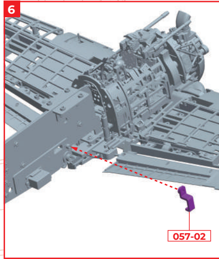
Fix the cockpit with 4 x screws 049-03 that were removed in STEP 2. Fit the gear cover 057-02 that came with stage 57 into the fuselage frame.
