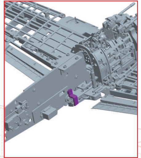
Fix the cockpit with 4 x screws 049-03 that were removed in STEP 2. Fit the gear cover 057-02 that came with stage 57 into the fuselage frame.
