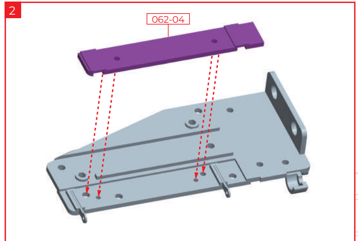
Align the screw holes, protrusions, and holes on the frame 062-03 and the hinge cover 062-04 and fit them together.
