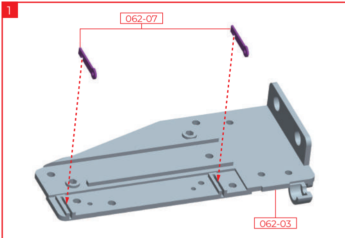
Fit the two hinges 062-07 into the frame 062-03 with the notches facing down.
