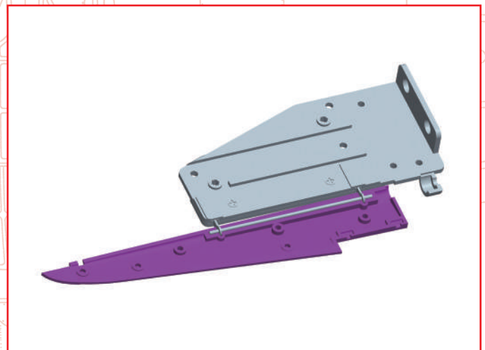
Fit two hinges 062-07 and shaft 062-09 into the groove on the lower surface 062-01 of the elevator (left).
