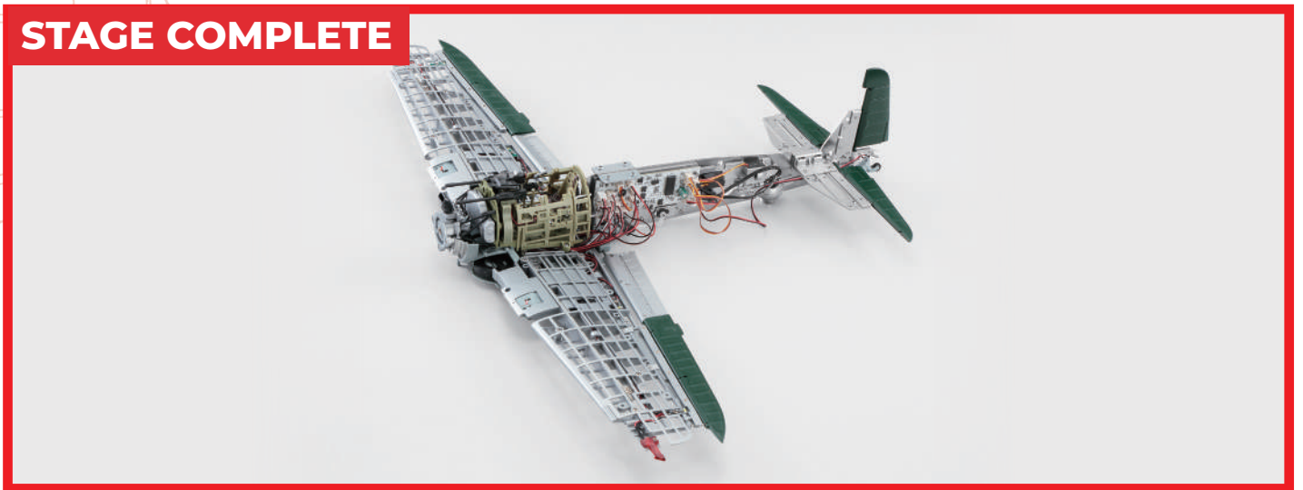
Fix the gear cover 057-02 in place with the screw 057-06 that came with stage 57.
