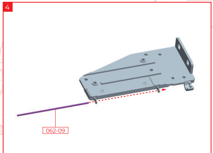
Thread the shaft 062-09 through the two holes on the hinge 062-07.
