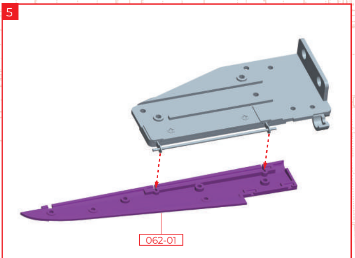
Fit two hinges 062-07 and shaft 062-09 into the groove on the lower surface 062-01 of the elevator (left).
