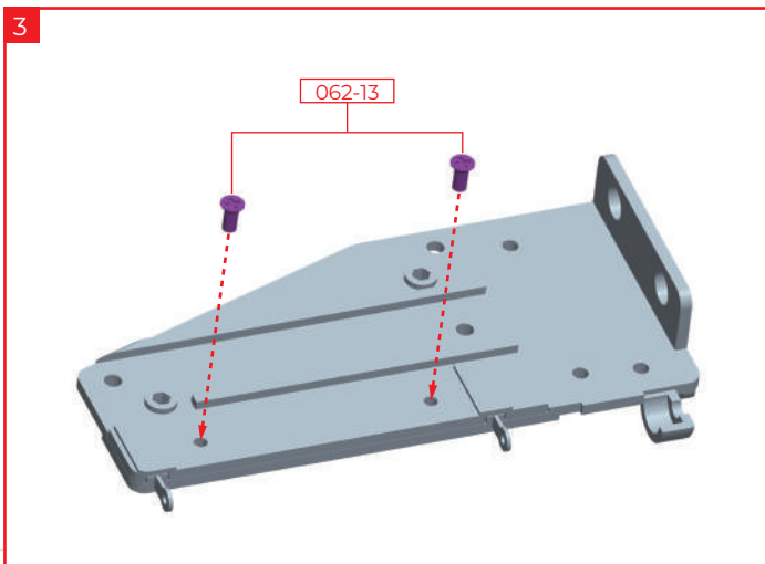
Fix the hinge cover 062-04 in place using 2 x screws 062-13.
